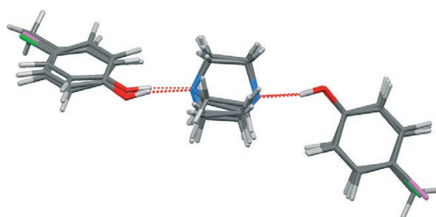
Figure 2. Superposition of the trimolecular assemblies in the binary cocrystals ClCl , MeMe , and BrBr . Dashed lines show the O–H...N hydrogen bonds. C gray, H white, N blue, O red, Cl green, Br pink.
